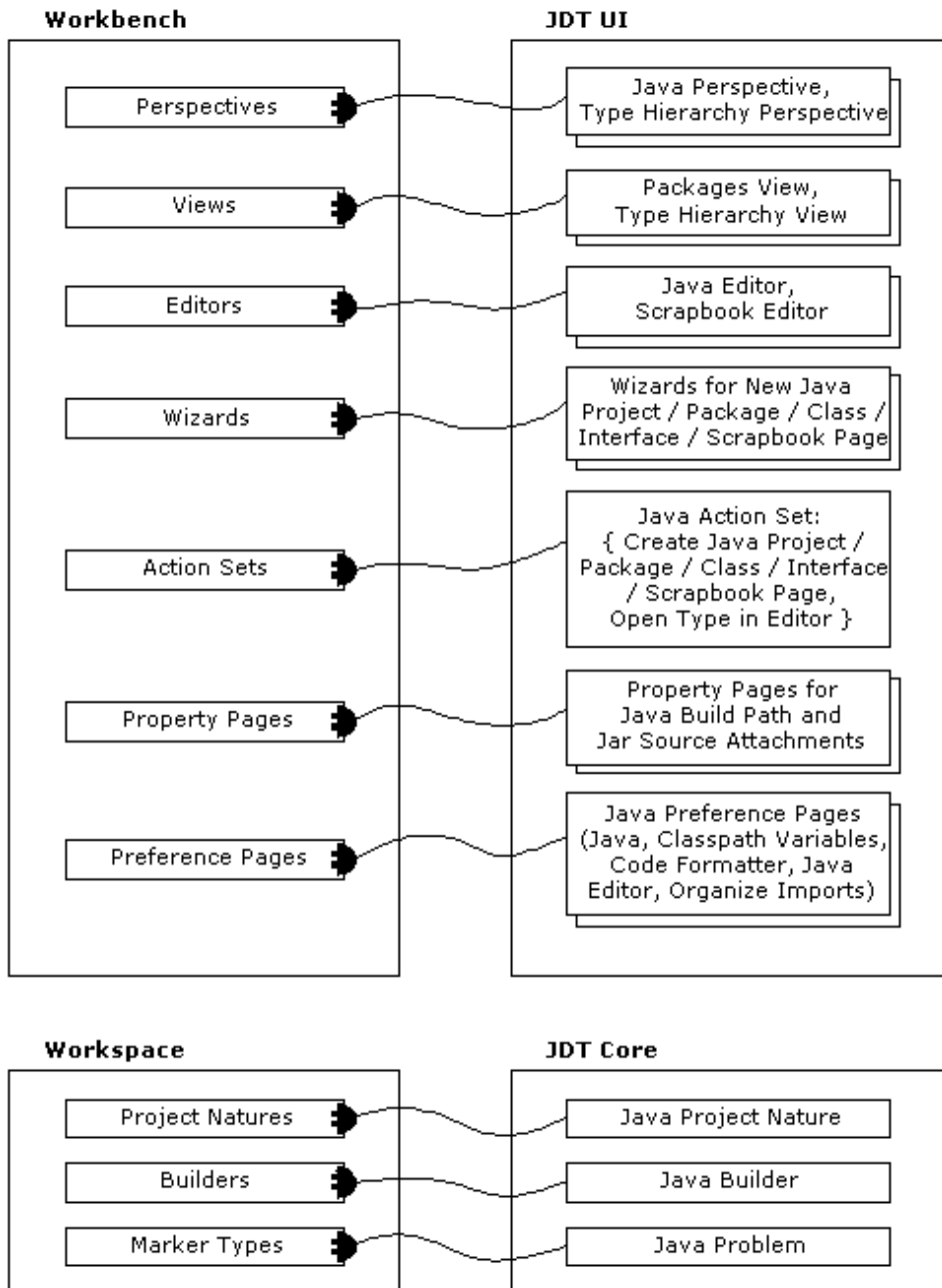
Figure 5 - Key connections between JDT and Eclipse Platform.
